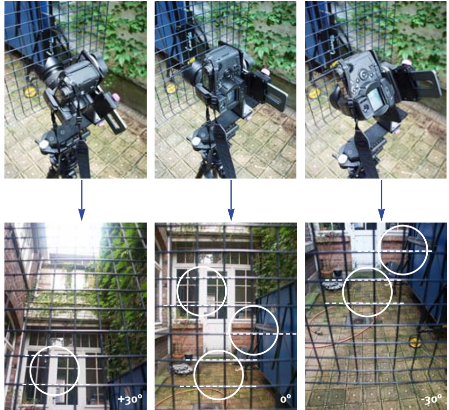
Here, the camera is misaligned. The tilting point is simply 10 mm behind the entrance pupil. Note the subtle shifts between the background and the horizontals of the grid (window frame, water hose, window sill, etc.).
